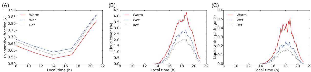
FIGURE 10 (A) Evaporative fraction, (B) cloud cover, and (C) liquid water path for the Warm, Wet, and reference numerical experiments. 41 Cloud cover is calculated by projecting all clouds onto the surface. Cloud cover and liquid water path are averaged over the horizontal extent of the domain.
